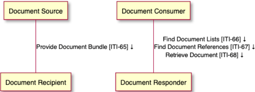
Figure 1 – IHE MHD Integration Profile Components and Transactions
