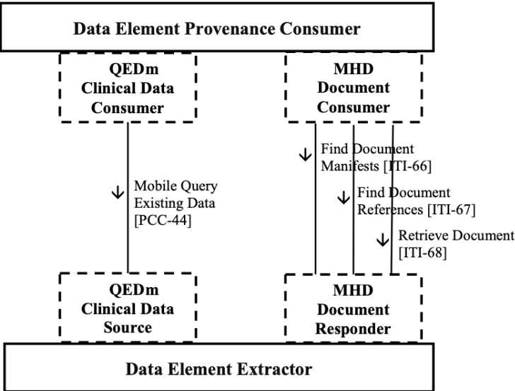
Figure 2 – IHE mXDE Integration Profile Components and Transactions
